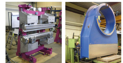
Revolver Mobile Undulator Carriages for the E.S.R.F. in France. Repeating Parallelism tolerance between the beams is 0,05 mm over 2,5 meters incl. beam rotation.
